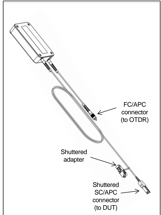
Figure 1. ELC-FCSC20MF1 launch cable
